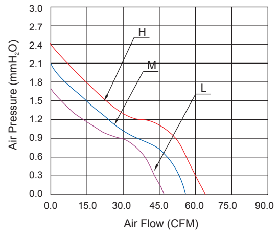
Performance Curves
