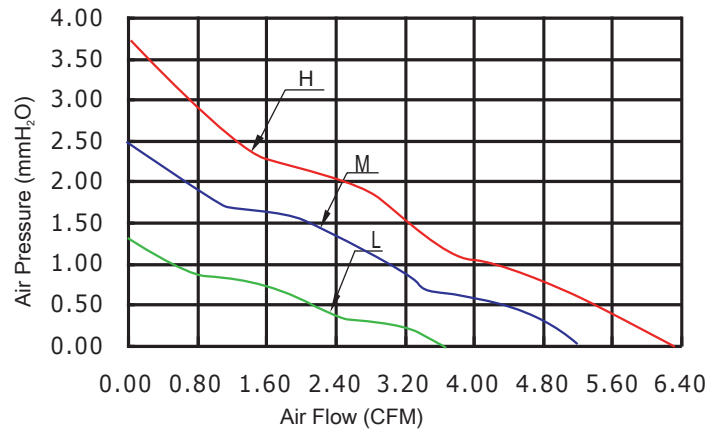
Performance Curves
